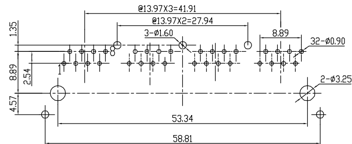
PC BOARD LAYOUT THICKNESS=1.6mm
